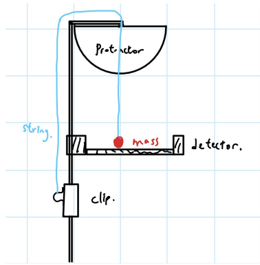
(a) Sketch of the Equipment Setup (With Detector)
